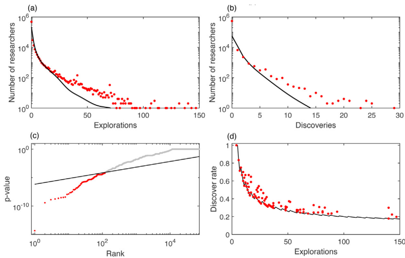
Fig. 2. Statistical significance of discoverers. We use the parameters F = 5 , K = 3 , f_p = 1.0(\%) , and T = 2006 as an example, that imply P_D = 7.6\% and P_E = 5.4\% . (a) Number of researchers who make different number of explorations (red dots); the black line represents the result under the null hypothesis, see Eq. (2). (b) Number of researchers who make different number of discoveries (red dots); the black line represent the result under the null hypothesis. (c) Author p-values obtained with Eq. (3) and the Benjamini-Hochberg procedure to control the False Discovery Rate. The solid line is \alpha r/N where N is the number of all active authors who made at least one exploration under the above parameter setting at T (here N = 72931 ), r is the author rank (the x-axis), and \alpha is the FDR level (we choose 5%). The dots below the line mark the authors who significantly deviate from the null hypothesis (red symbols); in this case, 124 discoverers are identified whose p-values are below p_m = 8.9 \times 10^{-5} . (d) The discovery rate ( D_i/E_i ) of the identified discoverers. The solid line shows the smallest discovery rate that would suffice to achieve the p-value under p_m at a given number of explorations.
